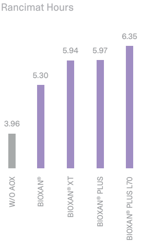
Rancimat Test at 110°C Sunflower Oil + AOX (1000ppm)
