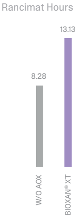
Rancimat Test at 90°C Rosehip Oil + AOX (1000ppm)
